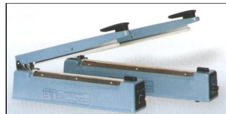
FS-300 12", 3mm, 430w, 11lbs. FS-400 16", 3mm, 600w, 15lbs.
