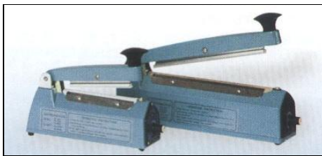
FS-100 4", 2mm, 180w, 5lbs. FS-200 8", 2mm, 330w, 7lbs.
